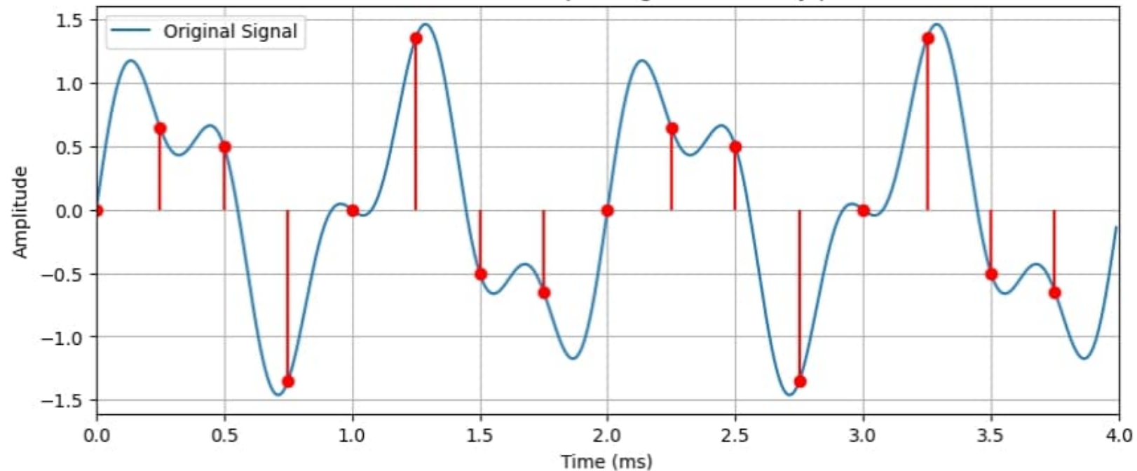
Reference and Sampled Signal - Below Nyquist
