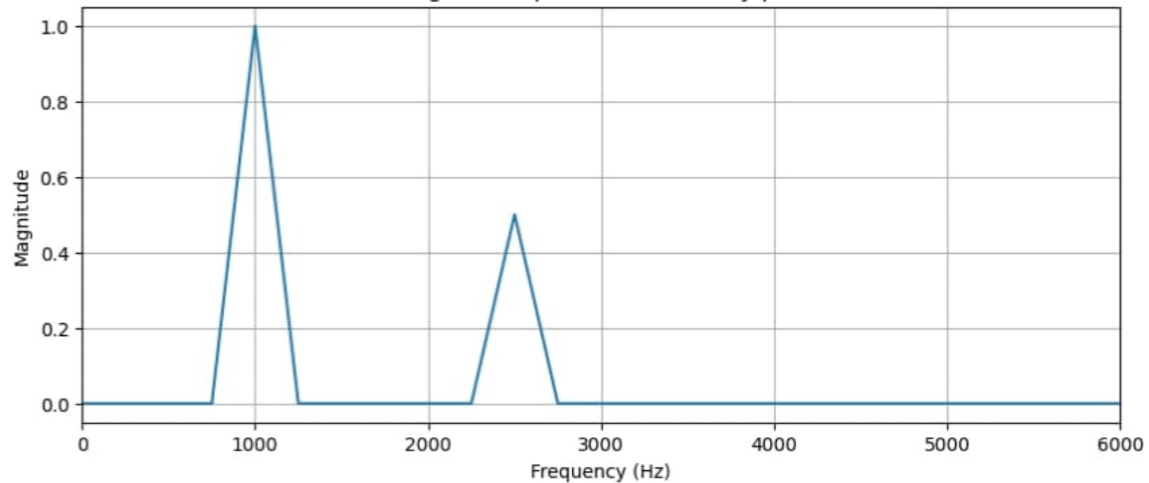
Magnitude Spectrum - Below Nyquist
