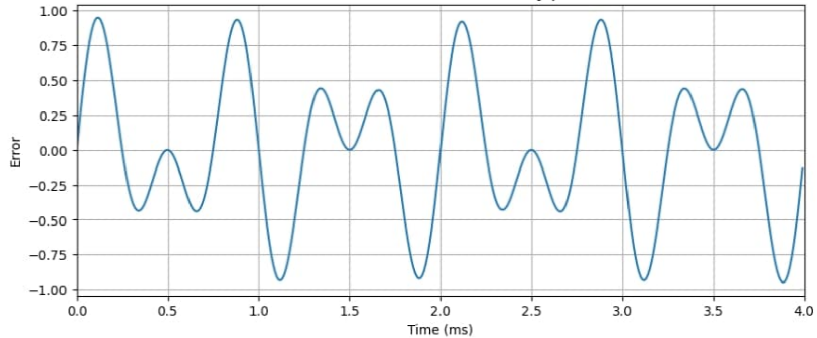
Reconstruction Error - Below Nyquist
