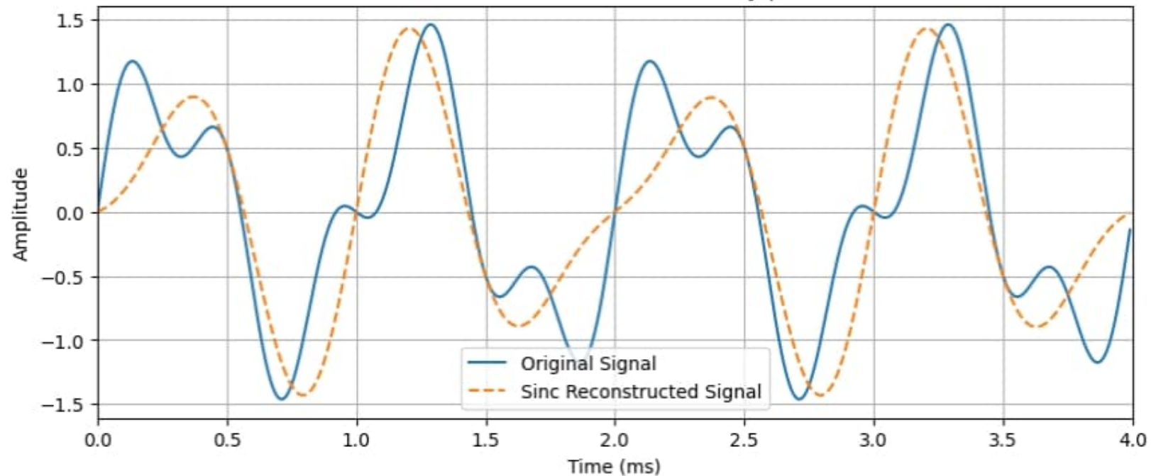
Sinc Reconstruction - Below Nyquist
